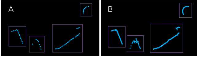
Figure 2. Each LIDAR rotational pass is slightly misaligned. We exploit this property by integrating data from multiple rotational passes. (A) shows a scene from a single pass, while (B) is integrated from 16 passes. Objects left to right: Mineral spirits can, user hand flat on surface, hammer, and bowl.
