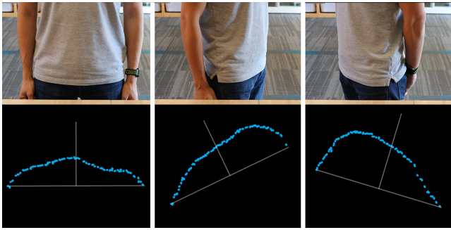
Figure 6. If SurfaceSight detects that a person is facing forwards, it also computes a body angle estimation. This extra contextual information could be used to e.g., enable voice interaction without a keyword when the user is sufficiently close and facing a device.
